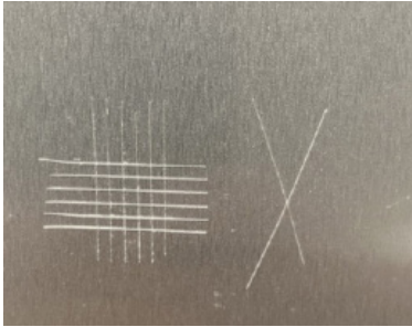
Cross-hatch and X-cut adhesion on aluminum
