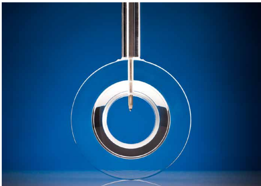
Flexible installation solutions for thermocouples and pressure sensors: specially developed sensor lens ring gaskets or conventional ring joint gaskets
