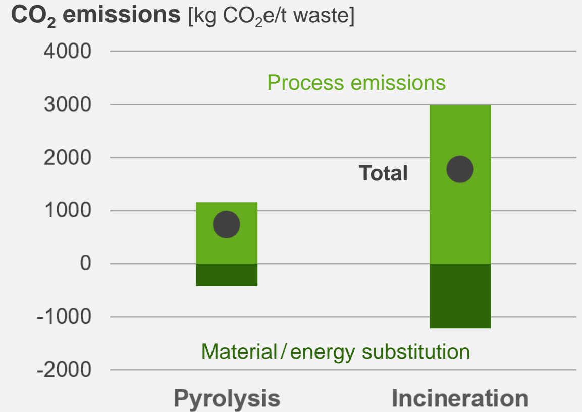
Fig. 1: Pyrolysis of 1t mixed plastic waste emits, in total, 739 kg CO 2 e. Incineration of 1t mixed plastic waste emits, in total, 1777 kg CO 2 e.
